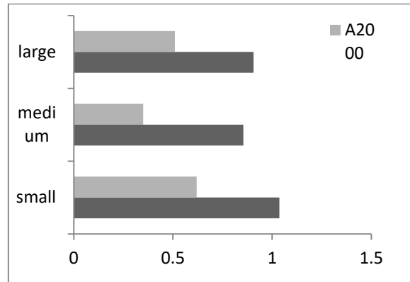
Figure 1. Energy intensity in Iranian industries at cluster level
